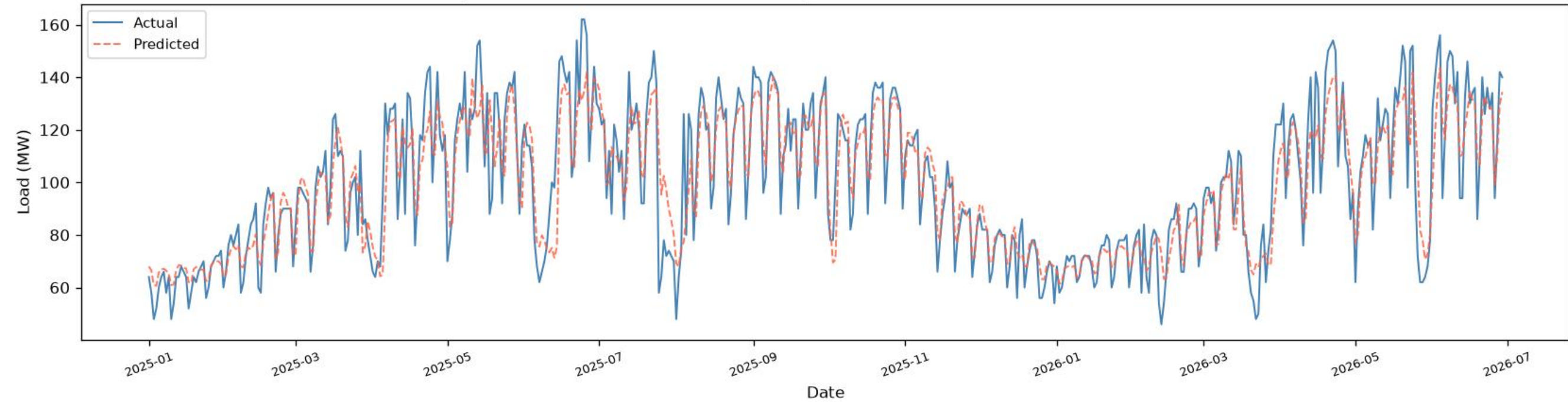
Gulshan | BiGRU+BiLSTM - TEST ( \geq 2025 ), one-day-ahead ( R^2=0.8260 , RMSE=11.67 , MAE=8.60 , n=536 )
