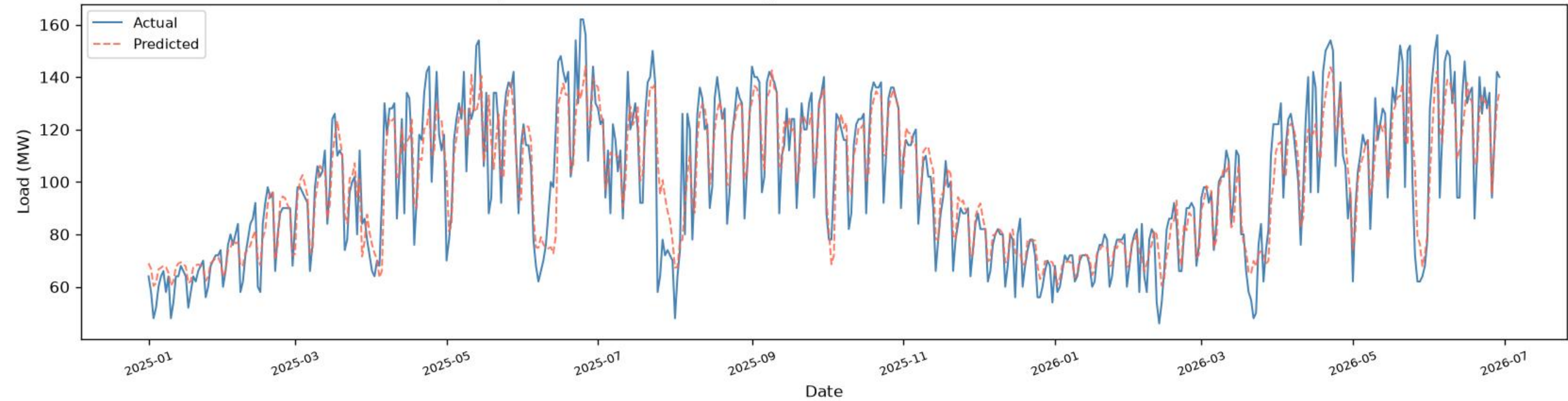
Gulshan | BiGRU - TEST ( \geq 2025 ), one-day-ahead ( R^2=0.8477 , RMSE=10.92 , MAE=8.04 , n=536 )
