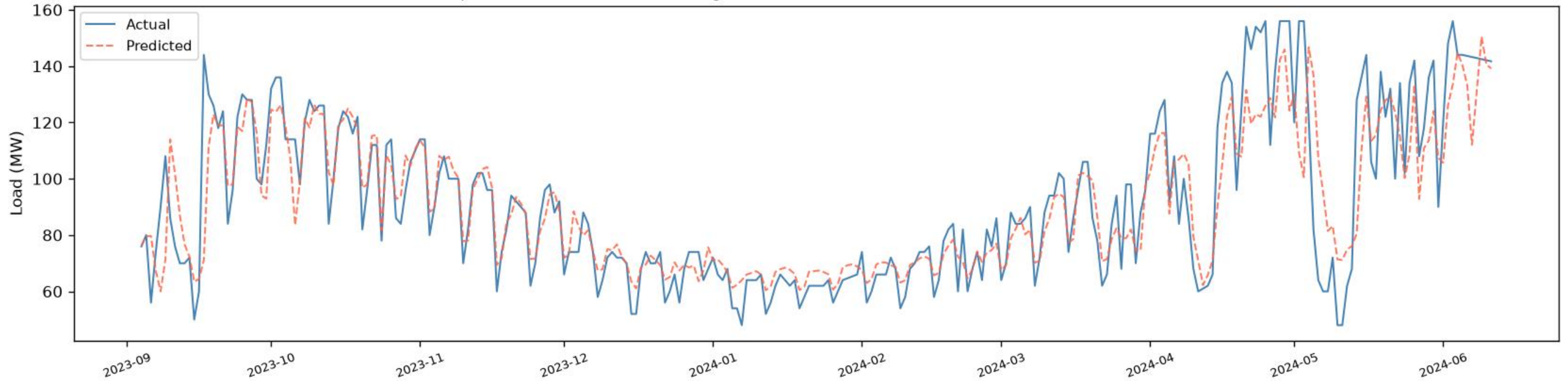
Gulshan | BiGRU - VALIDATION (chronological, before test) (R2=0.7587, RMSE=13.82, MAE=9.28, n=271)
