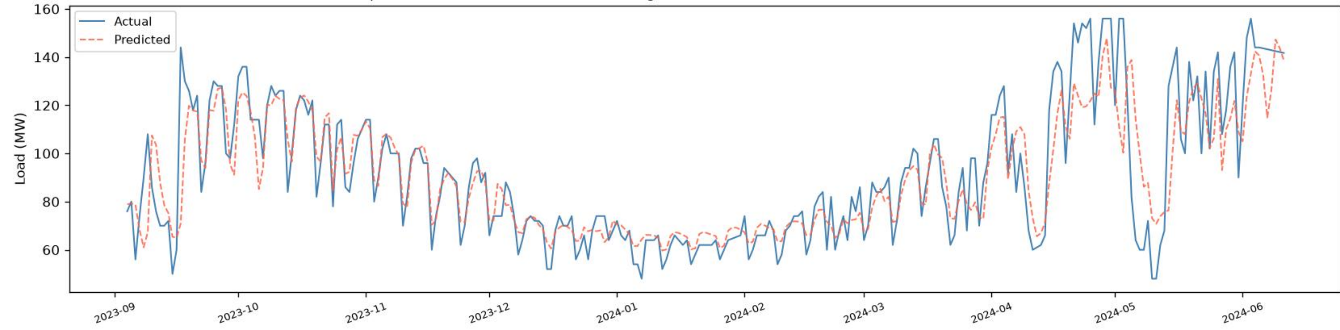
Gulshan | BiLSTM+BiGRU - VALIDATION (chronological, before test) ( R^2=0.7369 , RMSE=14.44 , MAE=9.58 , n=271 )
