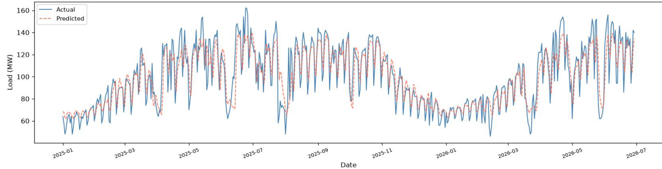
Gulshan | BiLSTM - TEST ( \geq 2025 ), one-day-ahead ( R^2=0.7848 , RMSE=12.98 , MAE=9.59 , n=536 )
