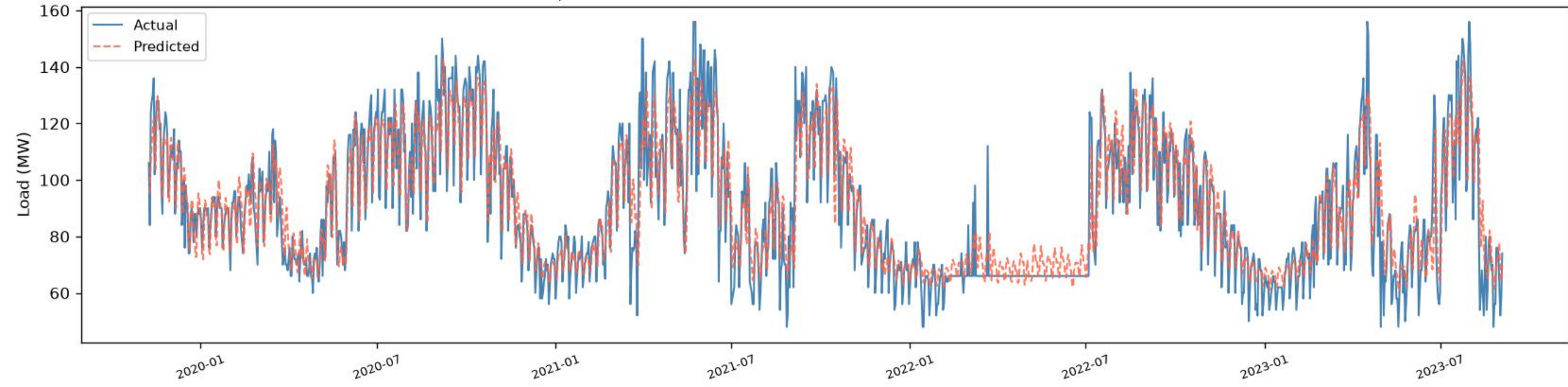
Gulshan | BiLSTM - TRAIN (fit block) ( R^2=0.8334 , RMSE=9.91, MAE=7.26, n=1351 )
