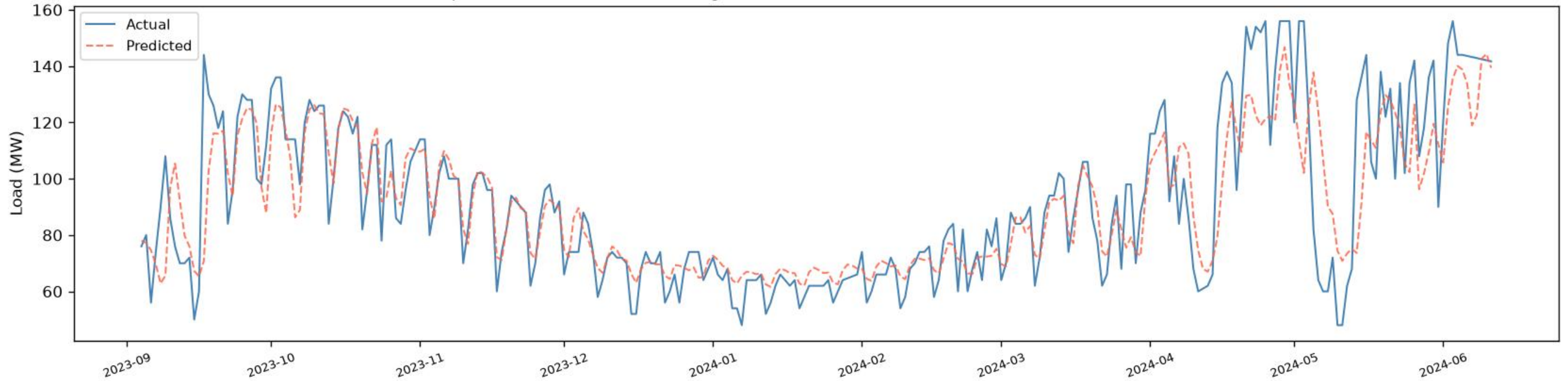
Gulshan | BiLSTM - VALIDATION (chronological, before test) (R2=0.7072, RMSE=15.23, MAE=10.22, n=271)
