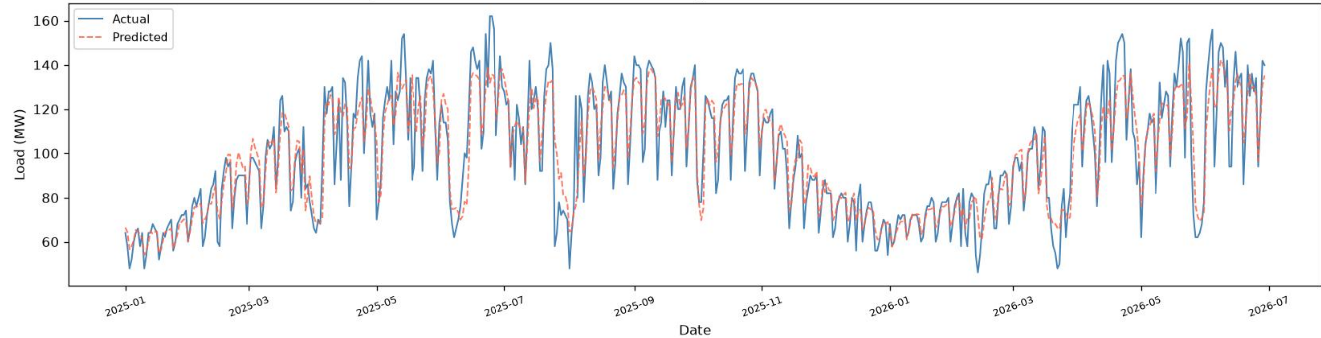
Gulshan | CNN+BiGRU+BiLSTM - TEST ( \geq 2025 ), one-day-ahead ( R^2=0.8630 , RMSE=10.36 , MAE=7.48 , n=536 )
