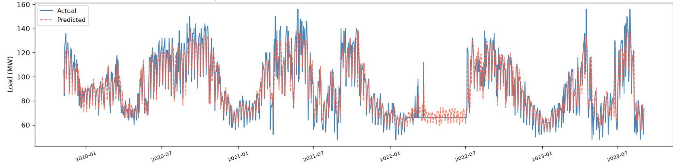
Gulshan | CNN+BiGRU+BiLSTM - TRAIN (fit block) (R2=0.8862, RMSE=8.19, MAE=5.78, n=1351)
