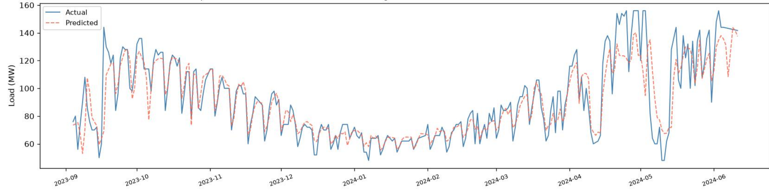
Gulshan | CNN+BiGRU+BiLSTM - VALIDATION (chronological, before test) ( R^2=0.7702 , RMSE=13.49, MAE=8.43, n=271 )
