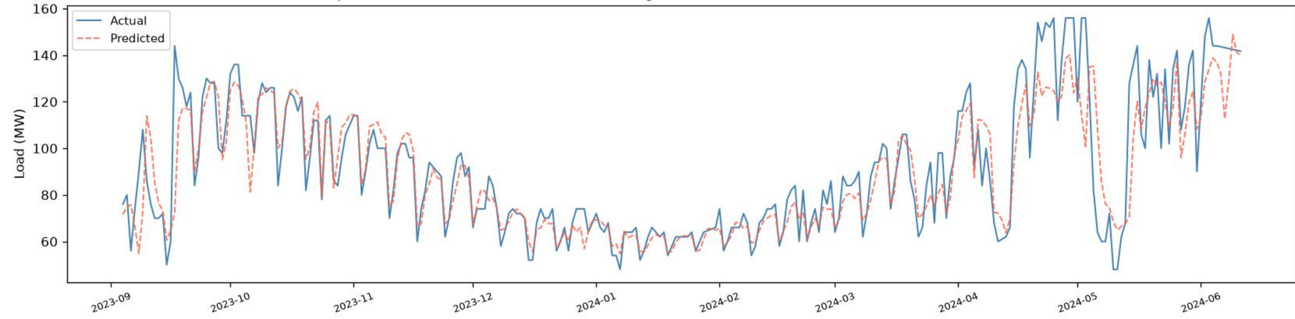
Gulshan | CNN+BiLSTM+BiGRU - VALIDATION (chronological, before test) ( R^2=0.7764 , RMSE=13.31, MAE=8.53, n=271)
