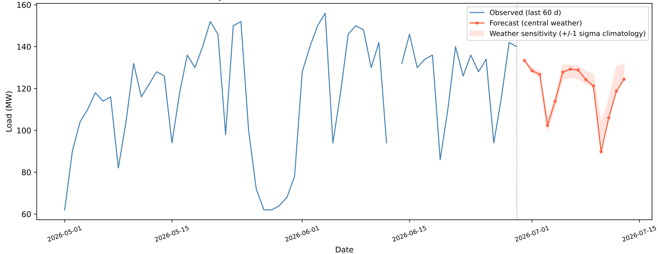
Gulshan - 14-day recursive forecast (CNN+BiLSTM+BiGRU), weather mode = forecast
