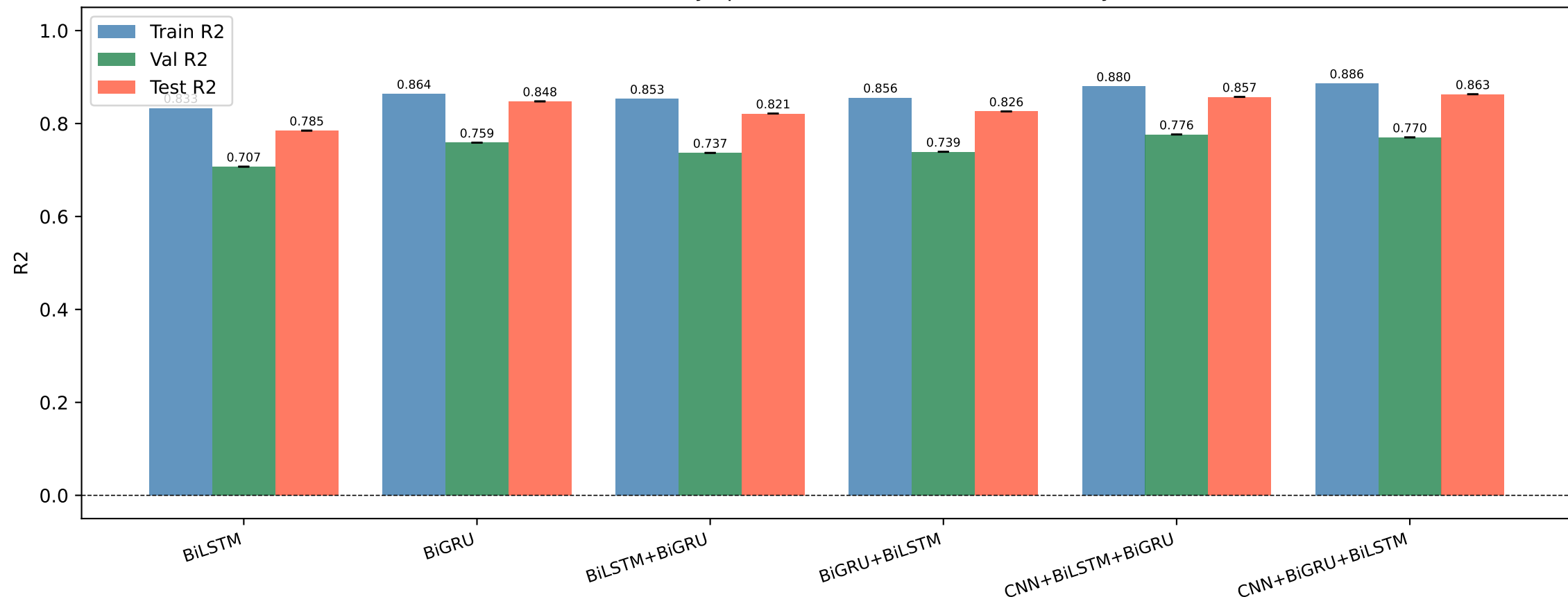
Gulshan - R2 by split (model selection uses VAL only)
