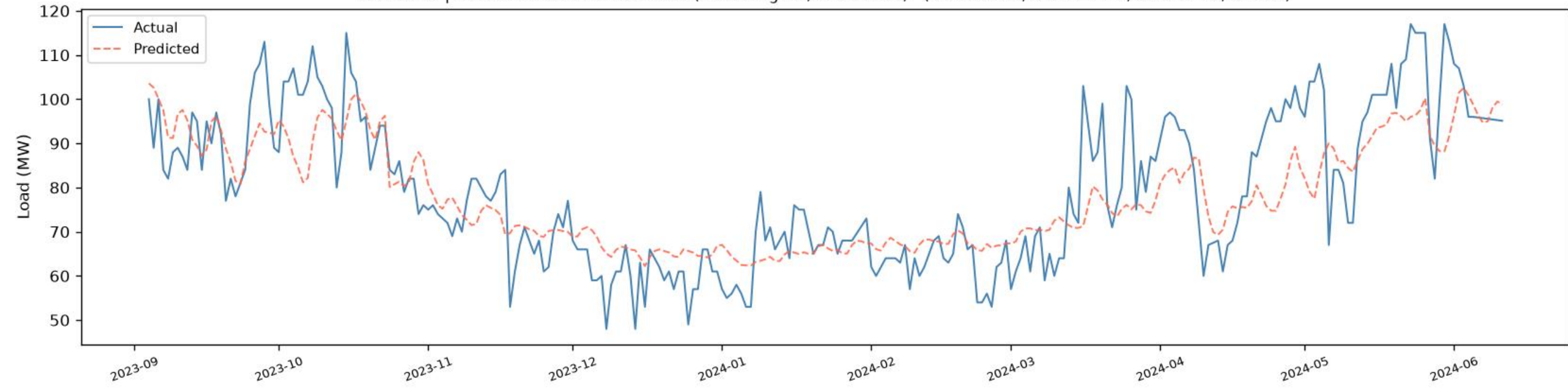
Hasnabad | BiGRU+BiLSTM - VALIDATION (chronological, before test) ( R^2=0.6528 , RMSE=9.96, MAE=7.74, n=271 )
