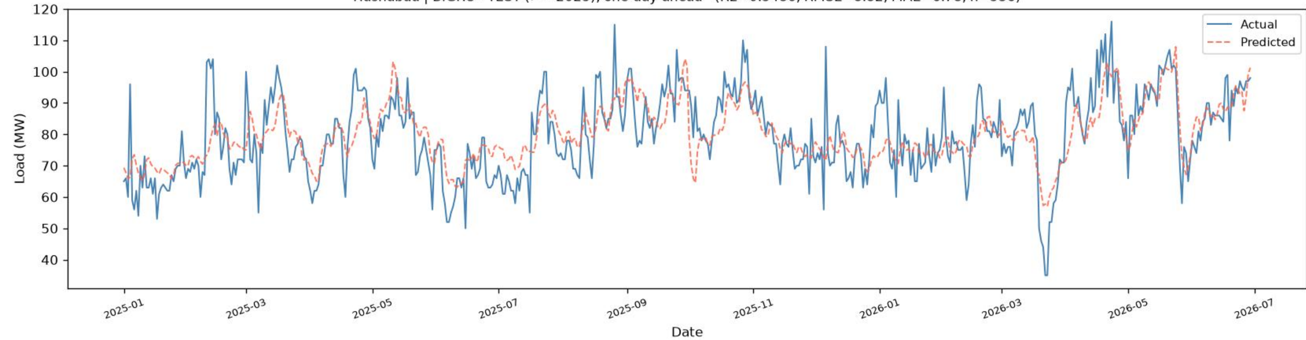
Hasnabad | BiGRU - TEST ( \geq 2025 ), one-day-ahead ( R^2=0.5486 , RMSE=8.82 , MAE=6.78 , n=536 )
