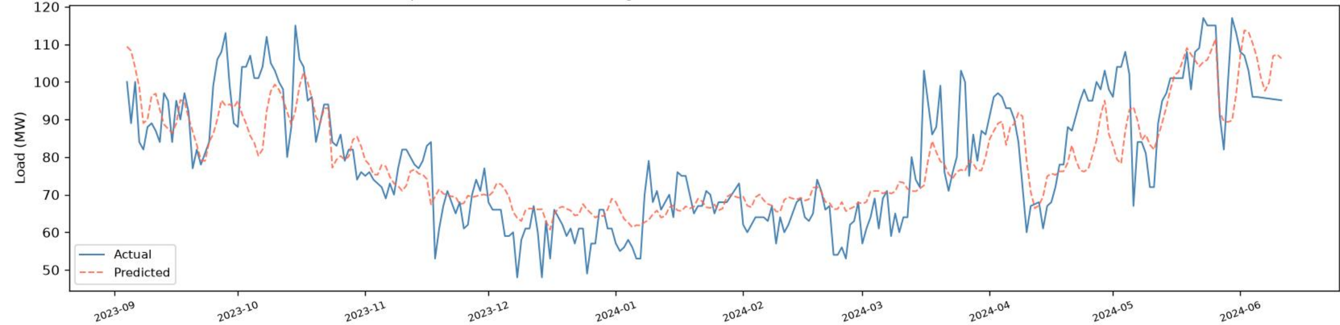
Hasnabad | BiGRU - VALIDATION (chronological, before test) (R2=0.6915, RMSE=9.38, MAE=7.20, n=271)
