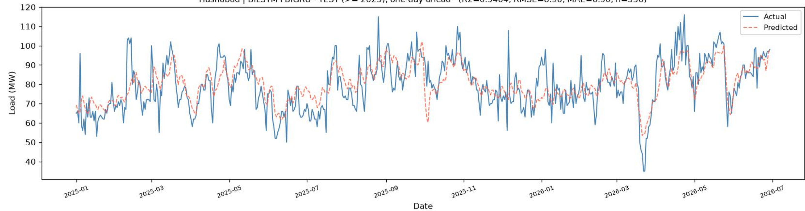
Hasnabad | BiLSTM+BiGRU - TEST ( \geq 2025 ), one-day-ahead ( R^2=0.5404 , RMSE=8.90 , MAE=6.90 , n=536 )
