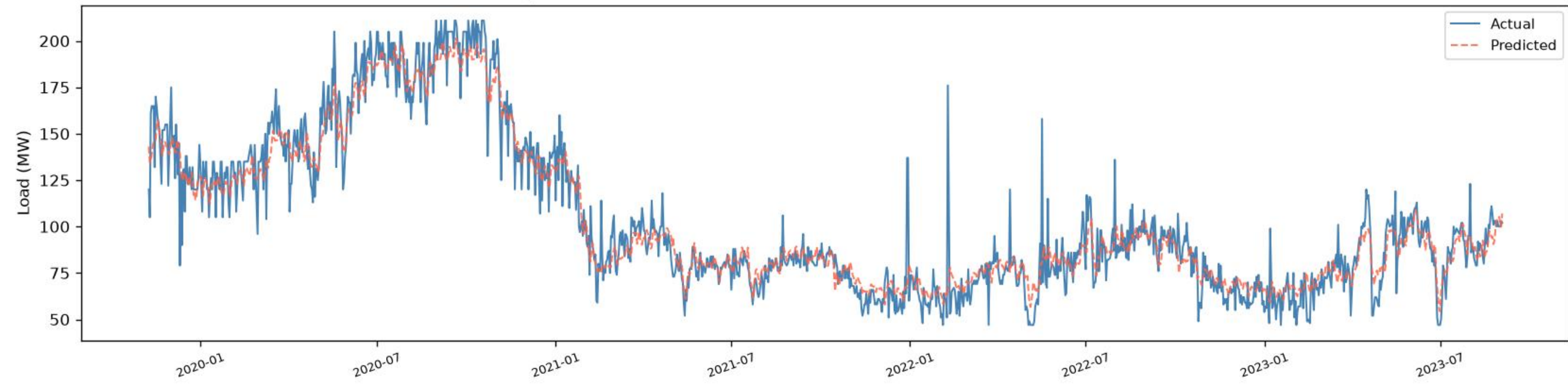
Hasnabad | BiLSTM+BiGRU - TRAIN (fit block) ( R^2=0.9284 , RMSE=11.30, MAE=8.07, n=1358)
