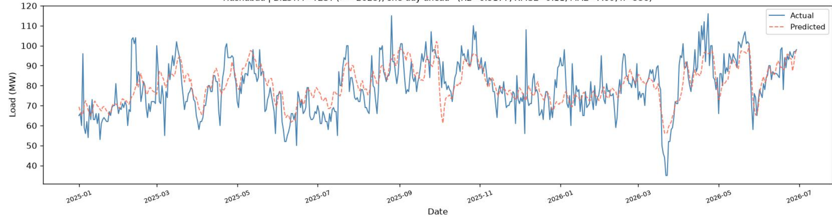
Hasnabad | BiLSTM - TEST ( \geq 2025 ), one-day-ahead ( R^2=0.5177 , RMSE=9.11 , MAE=7.09 , n=536 )
