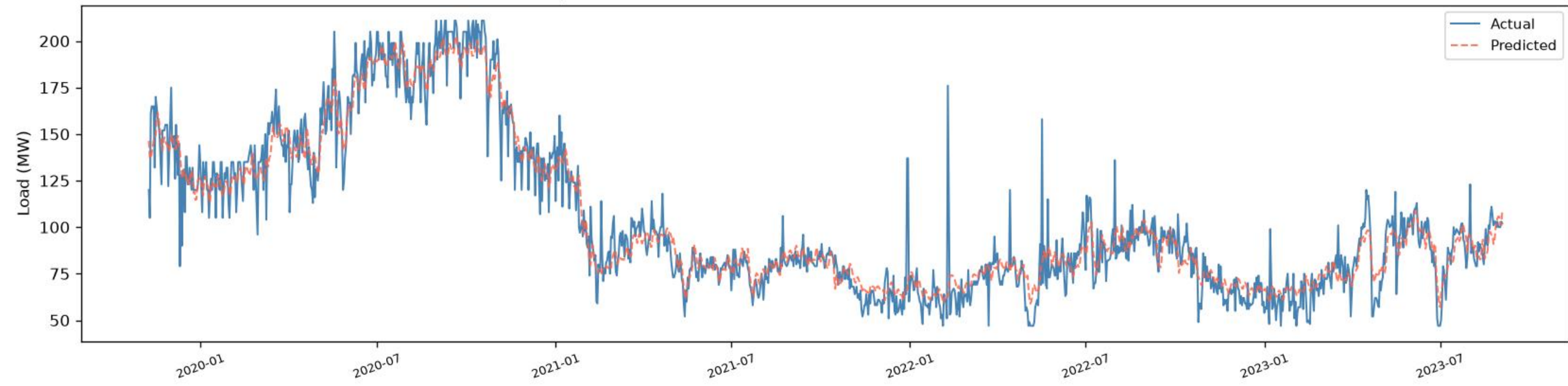
Hasnabad | BiLSTM - TRAIN (fit block) ( R^2=0.9279 , RMSE=11.34, MAE=8.06, n=1358)
