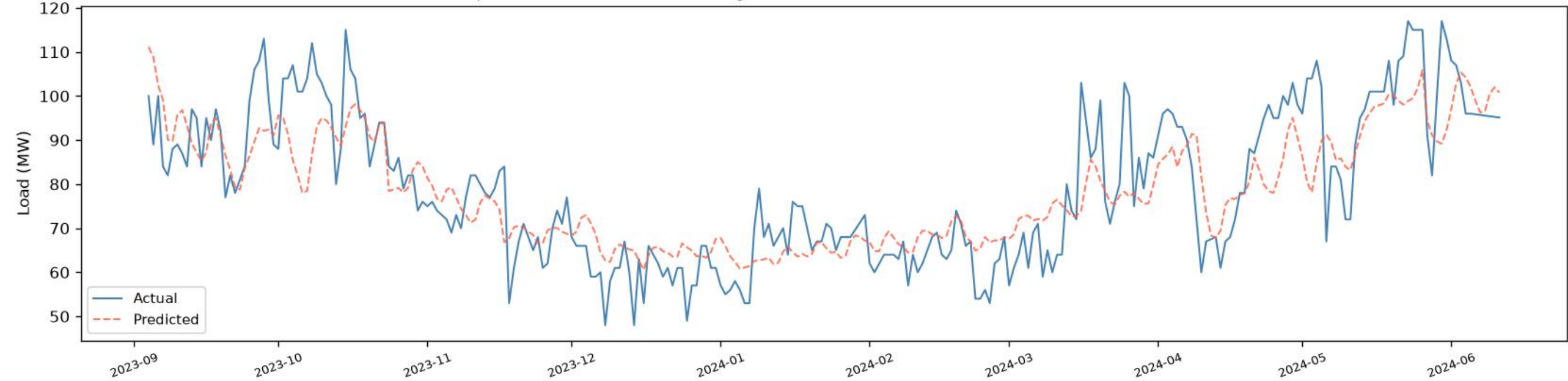
Hasnabad | BiLSTM - VALIDATION (chronological, before test) (R2=0.6768, RMSE=9.61, MAE=7.40, n=271)
