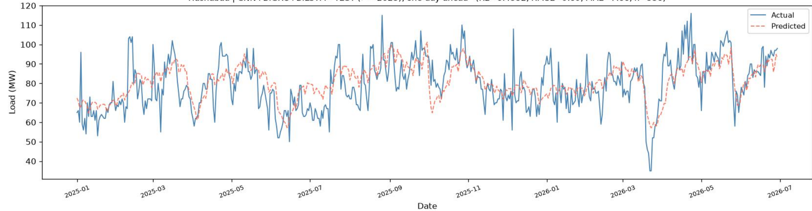
Hasnabad | CNN+BiGRU+BiLSTM - TEST ( \geq 2025 ), one-day-ahead ( R^2=0.4552 , RMSE=9.69 , MAE=7.66 , n=536 )
