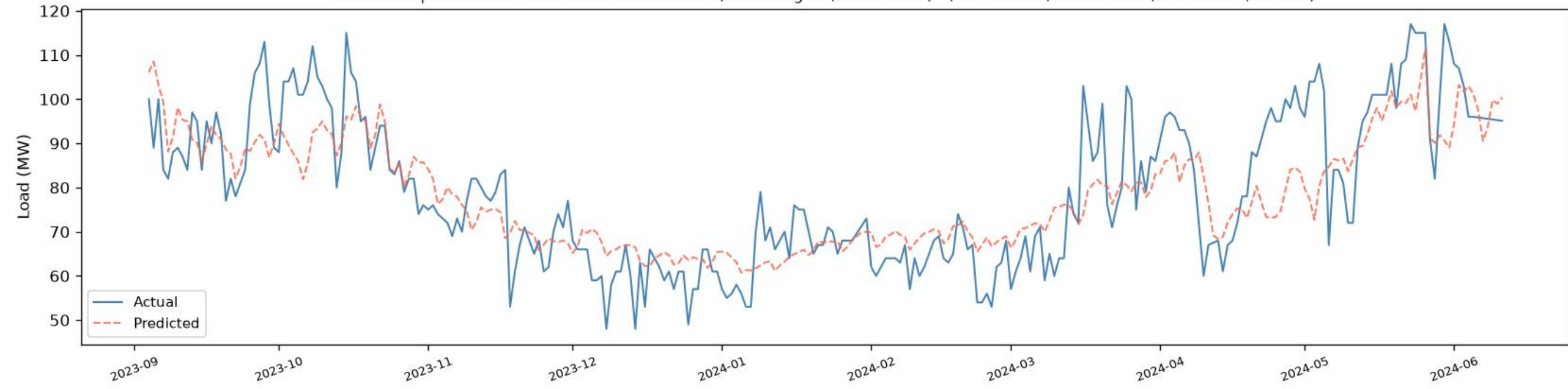
Hasnabad | CNN+BiGRU+BiLSTM - VALIDATION (chronological, before test) ( R^2=0.6534 , RMSE=9.95 , MAE=7.76 , n=271 )
