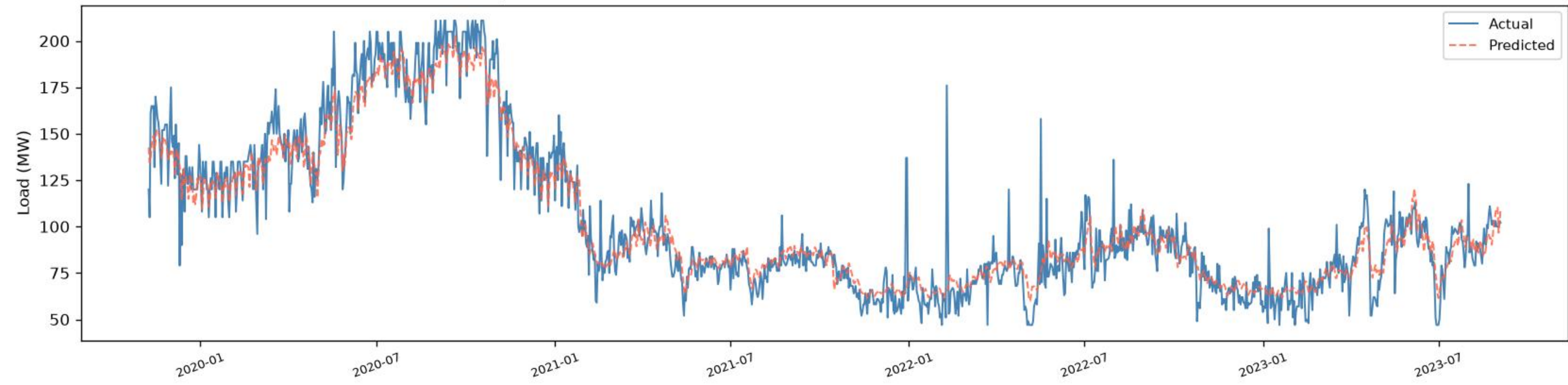
Hasnabad | CNN+BiLSTM+BiGRU - TRAIN (fit block) (R2=0.9255, RMSE=11.53, MAE=8.28, n=1358)
