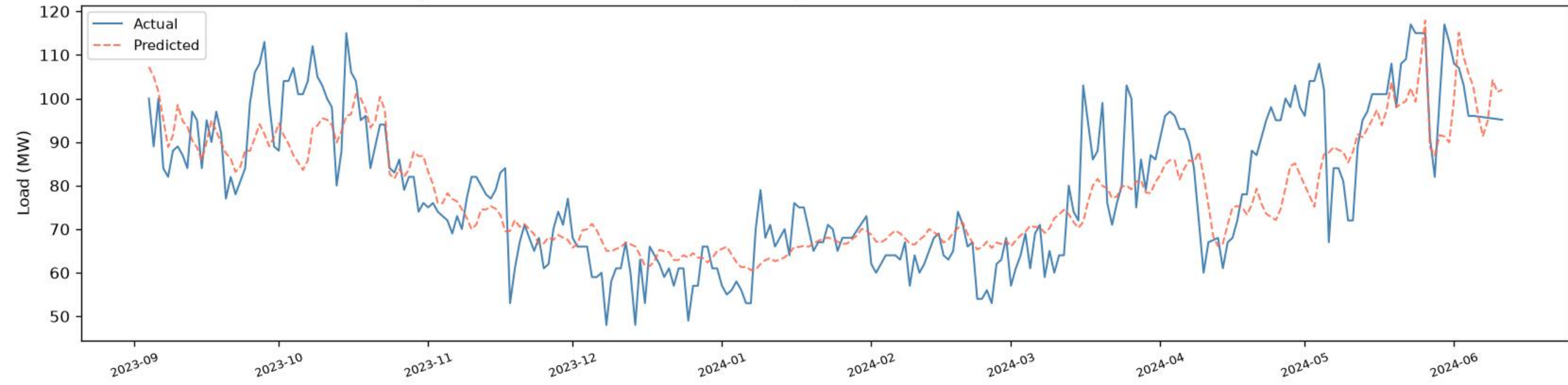
Hasnabad | CNN+BiLSTM+BiGRU - VALIDATION (chronological, before test) ( R^2=0.6663 , RMSE=9.76, MAE=7.66, n=271)
