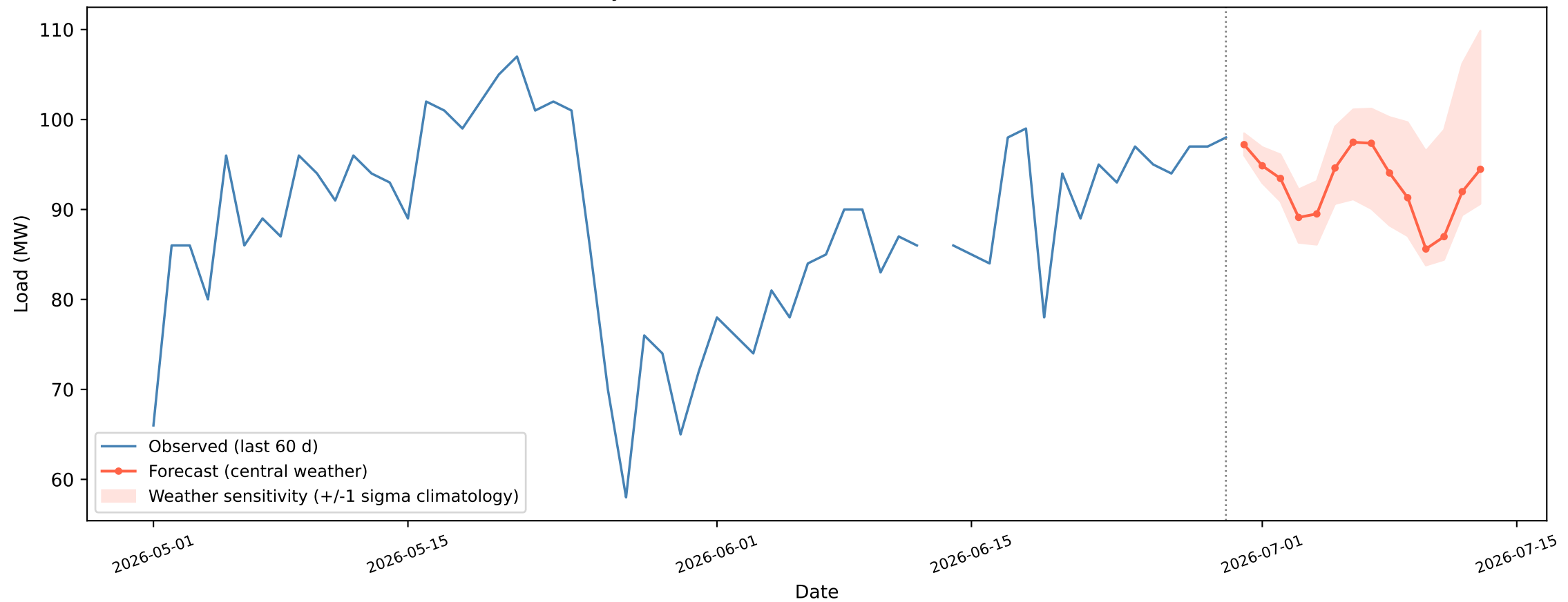
Hasnabad - 14-day recursive forecast (BiGRU), weather mode = forecast
