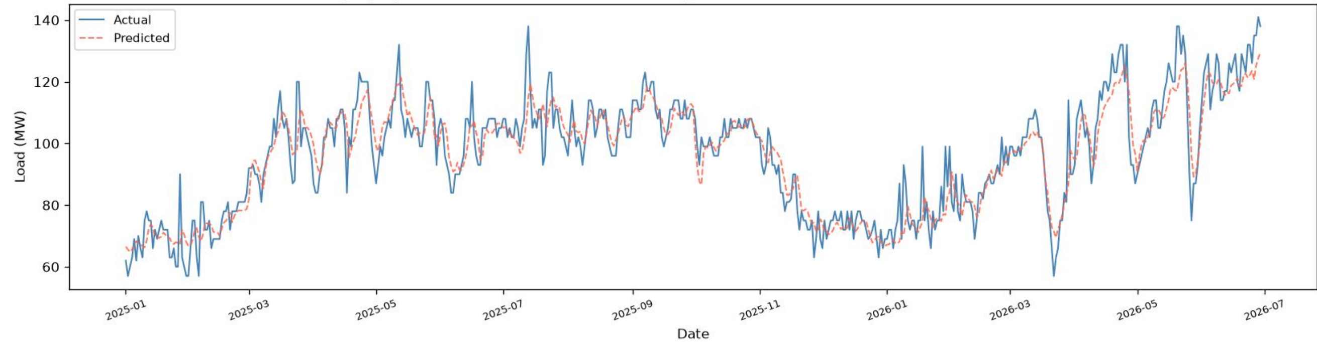
Kalyanpur | BiGRU+BiLSTM - TEST ( \geq 2025 ), one-day-ahead ( R^2=0.8586 , RMSE=6.88 , MAE=5.17 , n=536 )
