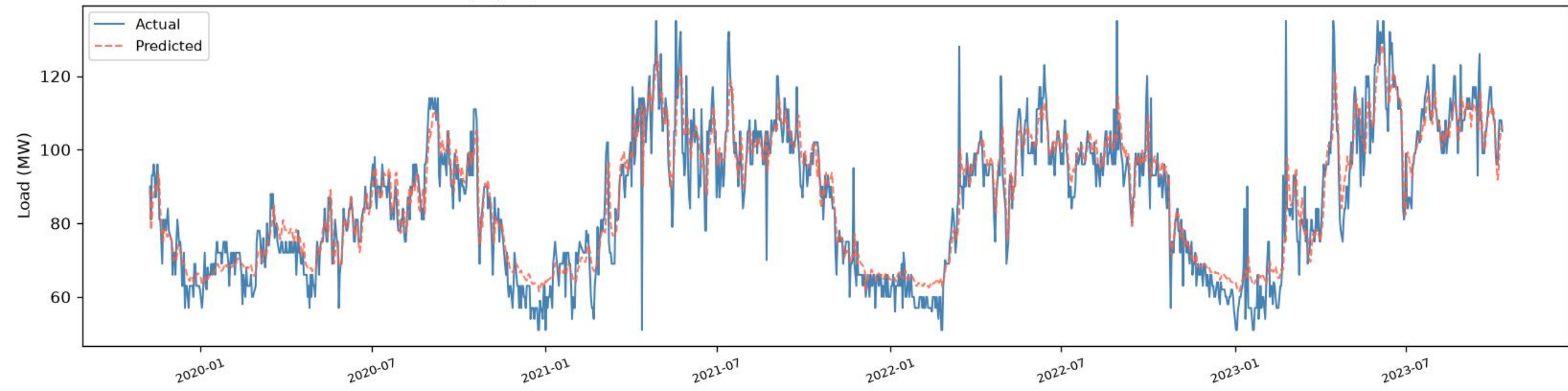
Kalyanpur | BiGRU+BiLSTM - TRAIN (fit block) (R2=0.8693, RMSE=6.83, MAE=4.89, n=1398)
