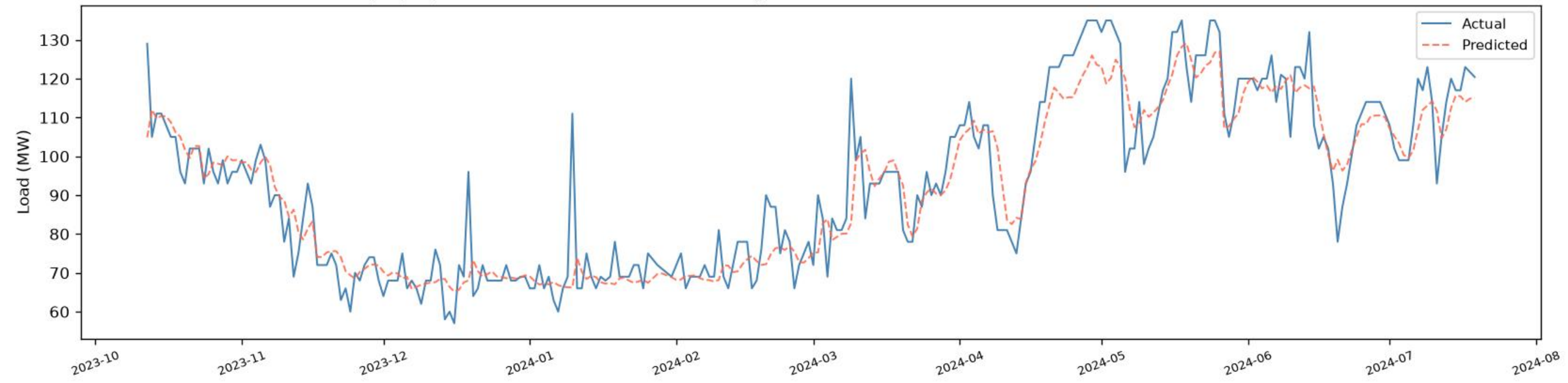
Kalyanpur | BiGRU+BiLSTM - VALIDATION (chronological, before test) ( R^2=0.8670 , RMSE=7.94 , MAE=5.49 , n=271 )
