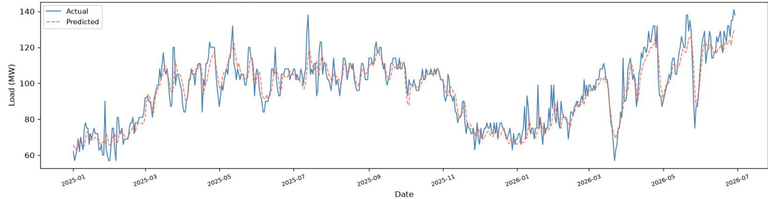
Kalyanpur | BiGRU - TEST ( \geq 2025 ), one-day-ahead ( R^2=0.8624 , RMSE=6.78 , MAE=5.08 , n=536 )
