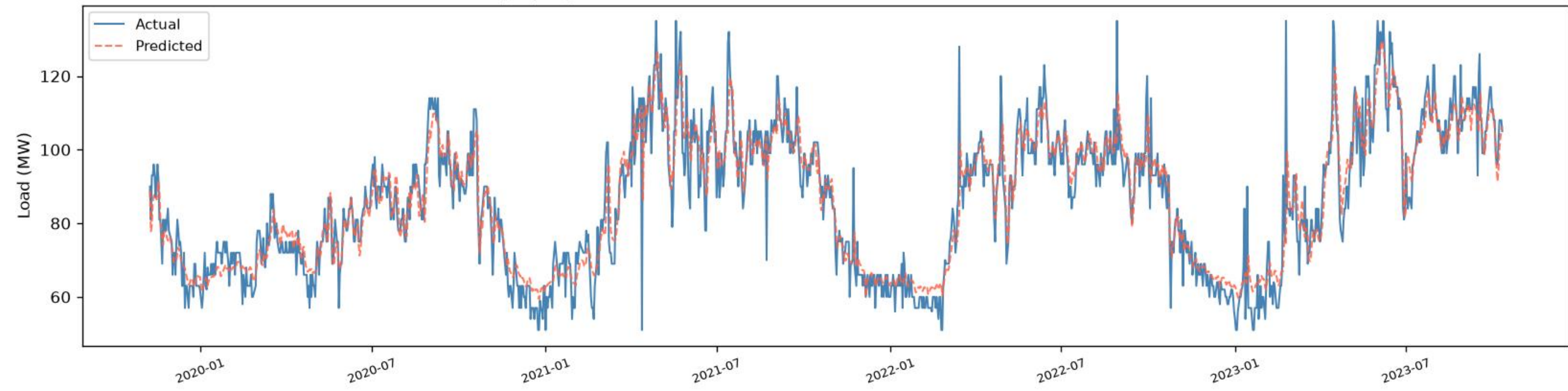
Kalyanpur | BiGRU - TRAIN (fit block) ( R^2=0.8773 , RMSE=6.62, MAE=4.63, n=1398)
