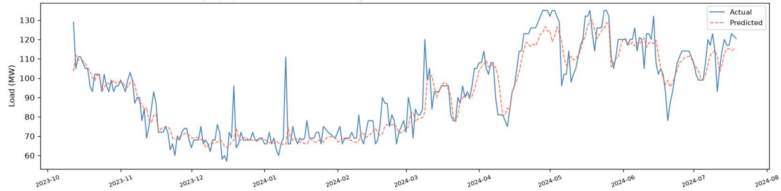
Kalyanpur | BiGRU - VALIDATION (chronological, before test) ( R^2=0.8719 , RMSE=7.79 , MAE=5.33 , n=271 )
