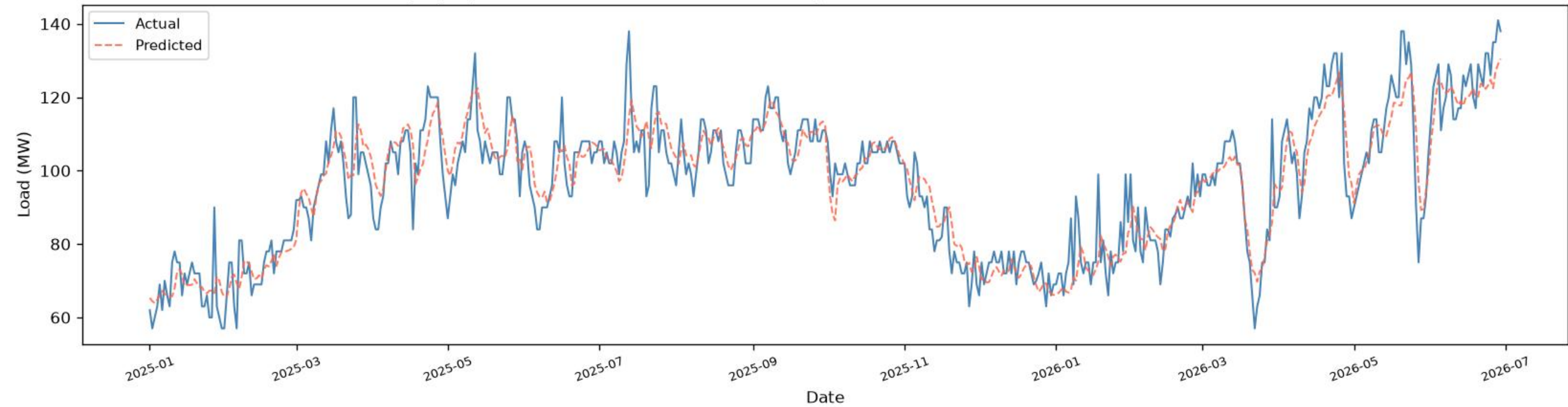
Kalyanpur | BiLSTM+BiGRU - TEST ( \geq 2025 ), one-day-ahead ( R^2=0.8556 , RMSE=6.95 , MAE=5.28 , n=536 )
