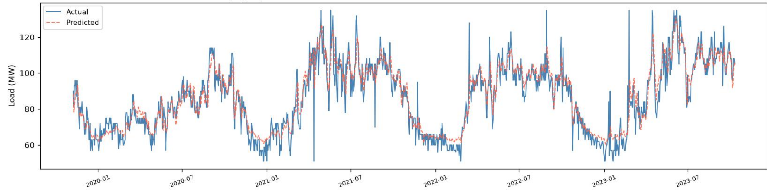
Kalyanpur | BiLSTM+BiGRU - TRAIN (fit block) (R2=0.8680, RMSE=6.87, MAE=4.88, n=1398)
