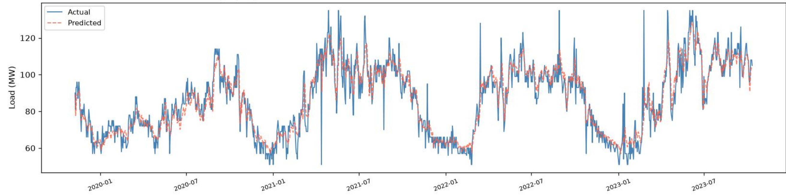
Kalyanpur | CNN+BiGRU+BiLSTM - TRAIN (fit block) (R2=0.8812, RMSE=6.52, MAE=4.55, n=1398)
