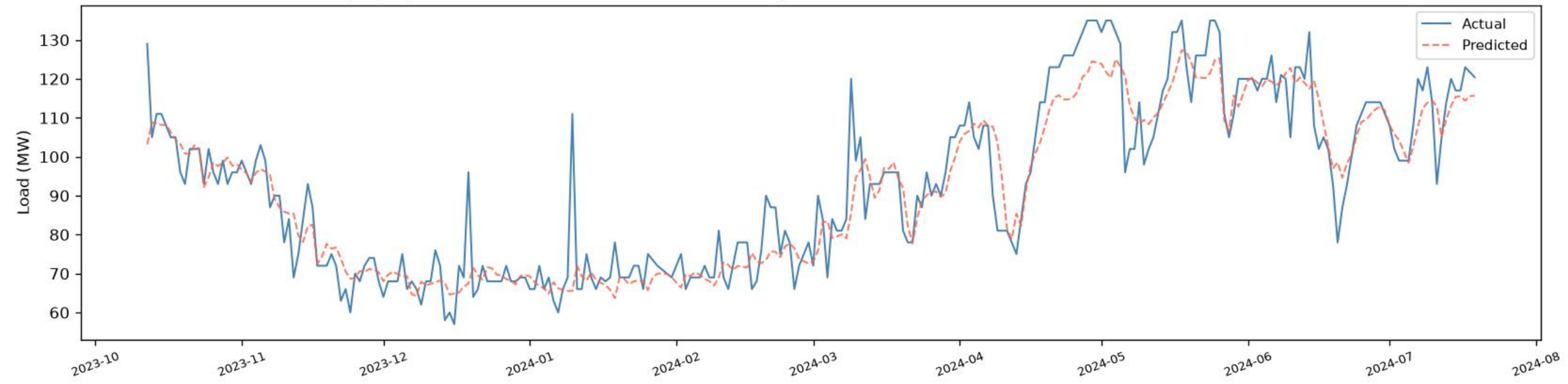
Kalyanpur | CNN+BiGRU+BiLSTM - VALIDATION (chronological, before test) ( R^2=0.8665 , RMSE=7.95 , MAE=5.50 , n=271 )
