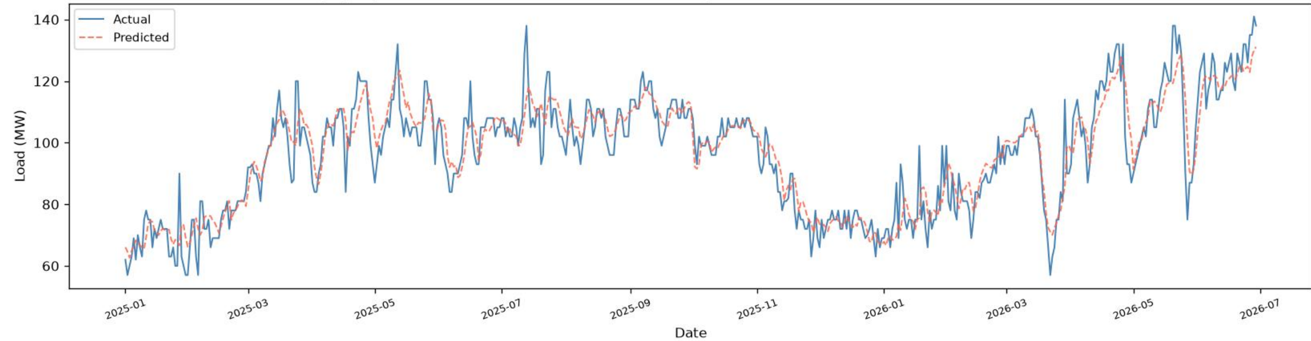
Kalyanpur | CNN+BiLSTM+BiGRU - TEST ( \geq 2025 ), one-day-ahead ( R^2=0.8517 , RMSE=7.04 , MAE=5.29 , n=536 )
