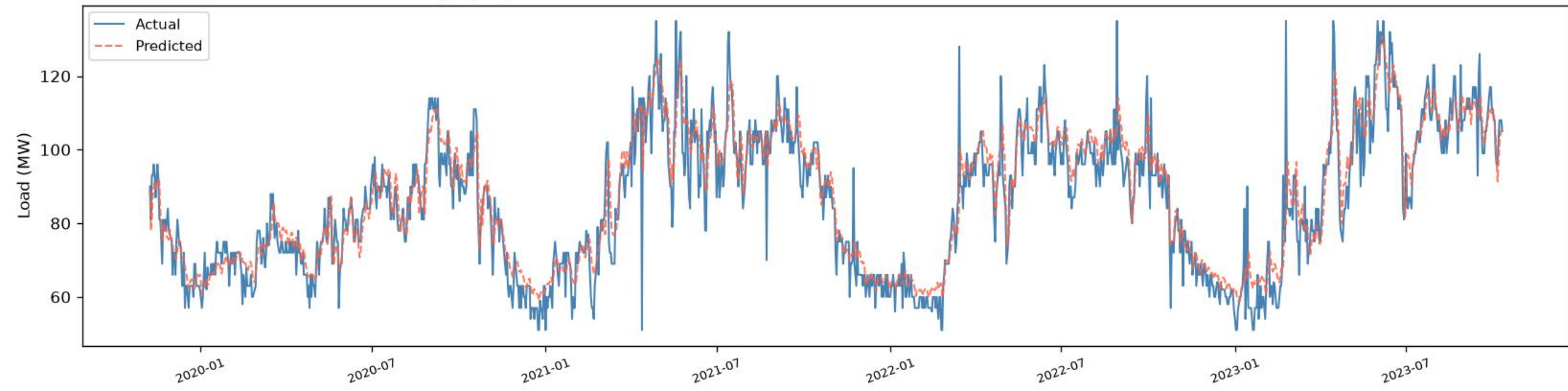
Kalyanpur | CNN+BiLSTM+BiGRU - TRAIN (fit block) (R2=0.8766, RMSE=6.64, MAE=4.70, n=1398)
