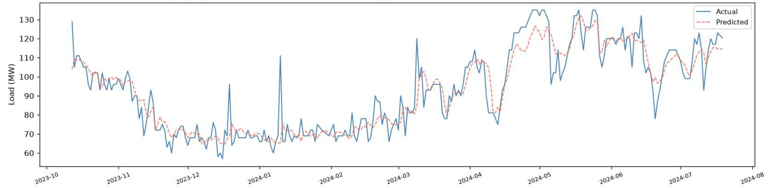
Kalyanpur | CNN+BiLSTM+BiGRU - VALIDATION (chronological, before test) ( R^2=0.8629 , RMSE=8.06 , MAE=5.54 , n=271 )
