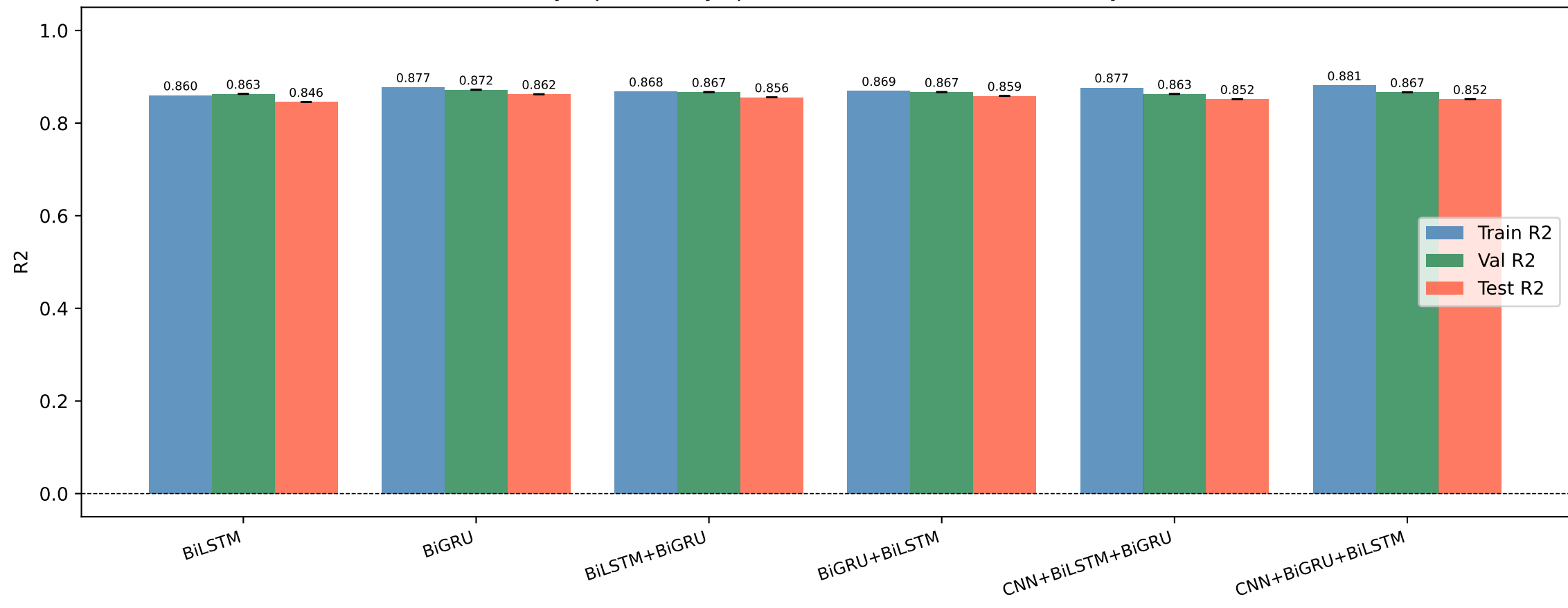
Kalyanpur - R2 by split (model selection uses VAL only)
