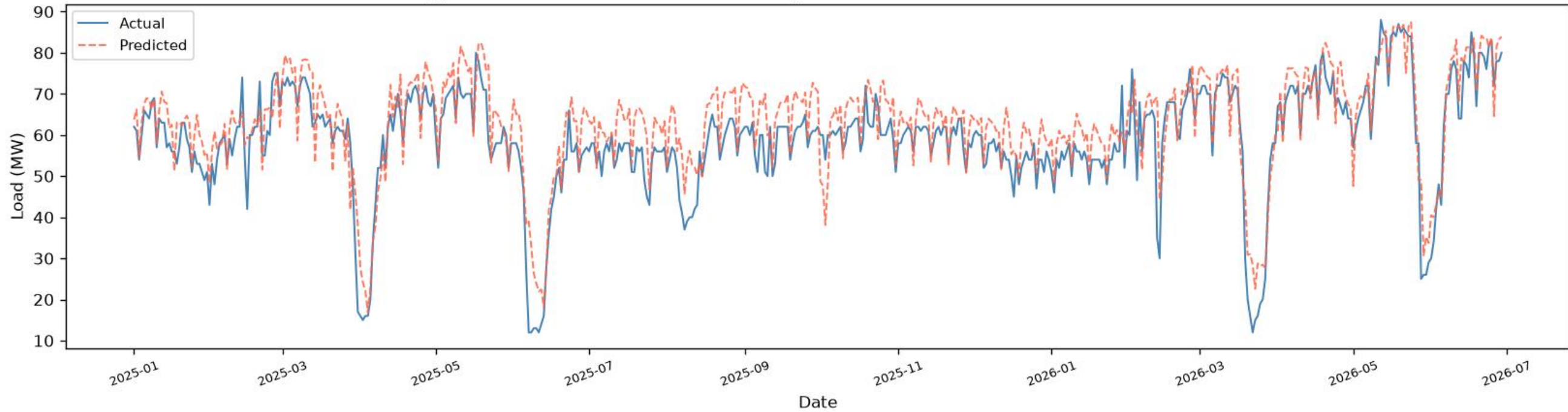
Lalbag | BiGRU+BiLSTM - TEST ( \geq 2025 ), one-day-ahead ( R^2=0.7299 , RMSE=7.01 , MAE=5.61 , n=527 )
