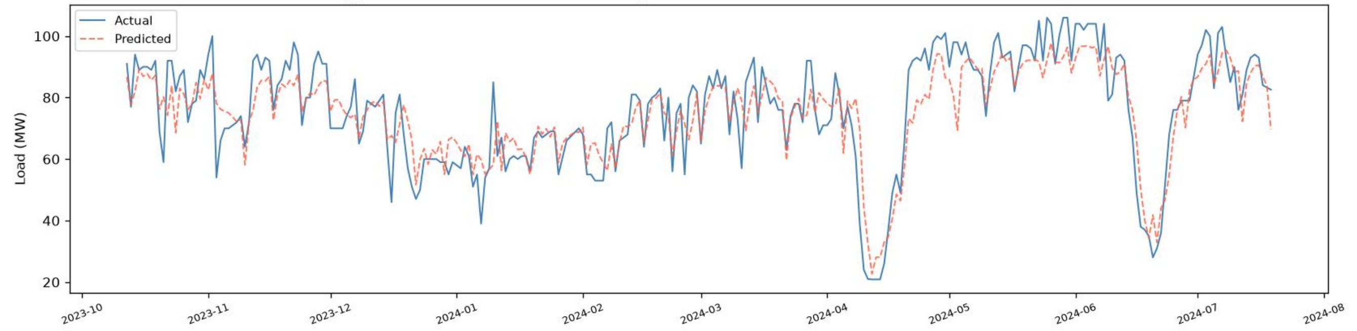
Lalbag | BiGRU+BiLSTM - VALIDATION (chronological, before test) ( R^2=0.7675 , RMSE=8.71 , MAE=6.71 , n=272 )
