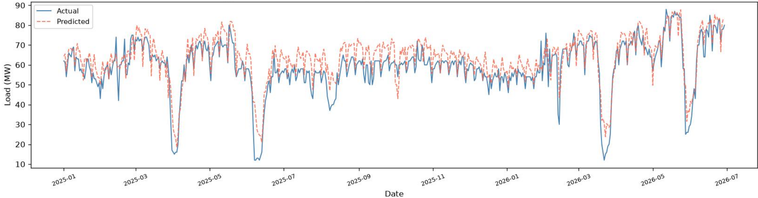
Lalbag | BiGRU - TEST ( \geq 2025 ), one-day-ahead (R2=0.7142, RMSE=7.21, MAE=5.77, n=527)
