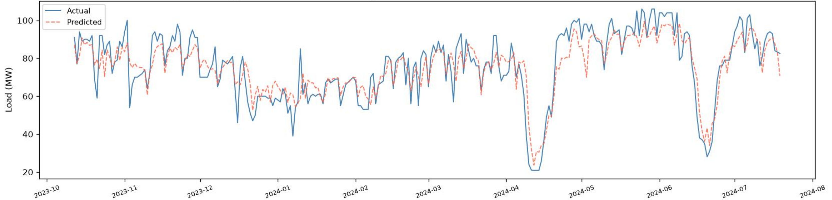
Lalbag | BiGRU - VALIDATION (chronological, before test) (R2=0.7725, RMSE=8.62, MAE=6.64, n=272)
