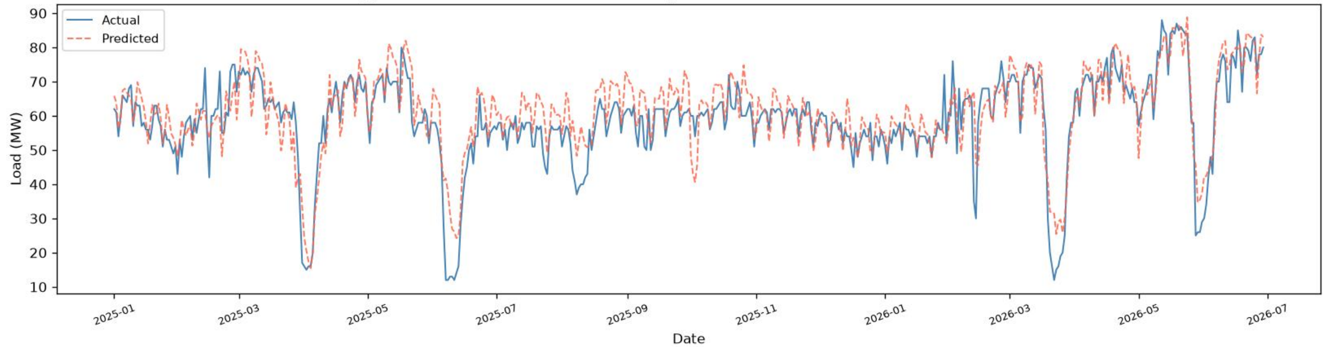
Lalbag | BiLSTM+BiGRU - TEST ( \geq 2025 ), one-day-ahead ( R^2=0.7482 , RMSE=6.77 , MAE=5.20 , n=527 )
