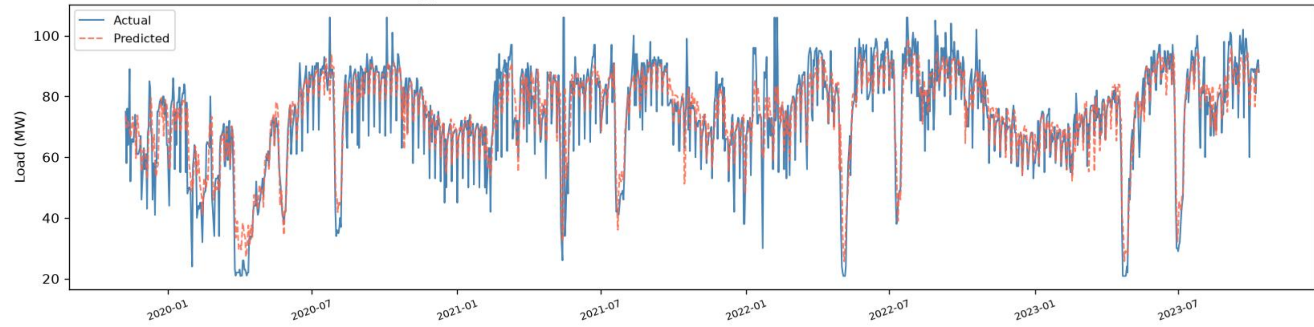
Lalbag | BiLSTM+BiGRU - TRAIN (fit block) ( R^2=0.7905 , RMSE=7.68, MAE=5.40, n=1398 )
