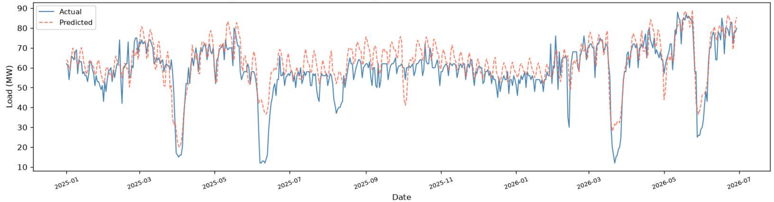
Lalbag | BiLSTM - TEST ( \geq 2025 ), one-day-ahead ( R^2=0.6413 , RMSE=8.08 , MAE=6.30 , n=527 )
