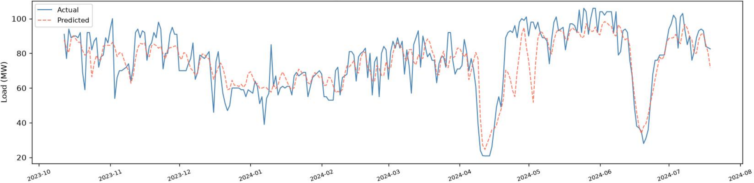
Lalbag | BiLSTM - VALIDATION (chronological, before test) (R2=0.6539, RMSE=10.63, MAE=8.00, n=272)
