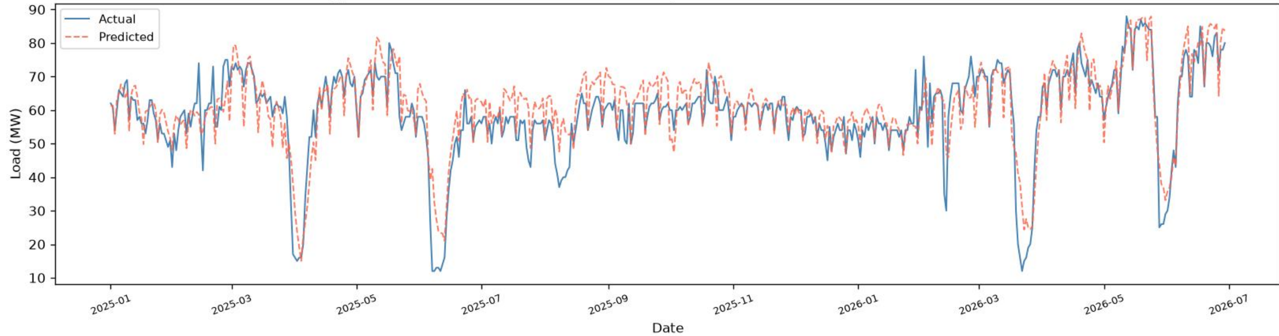
Lalbag | CNN+BiGRU+BiLSTM - TEST ( \geq 2025 ), one-day-ahead ( R^2=0.7576 , RMSE=6.64 , MAE=4.98 , n=527 )
