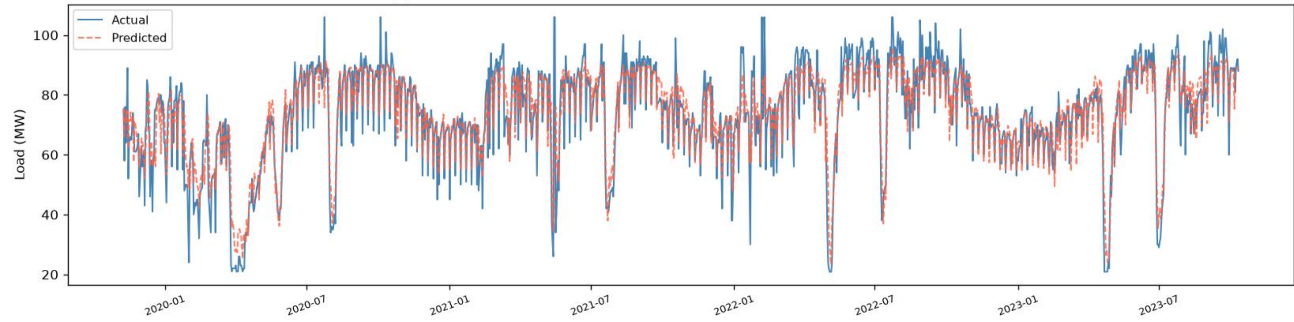
Lalbag | CNN+BiGRU+BiLSTM - TRAIN (fit block) (R2=0.8294, RMSE=6.93, MAE=4.71, n=1398)
